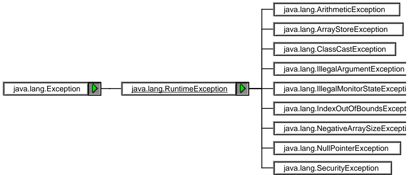
Figure 2.4. The Runtime Exception classes in Java
