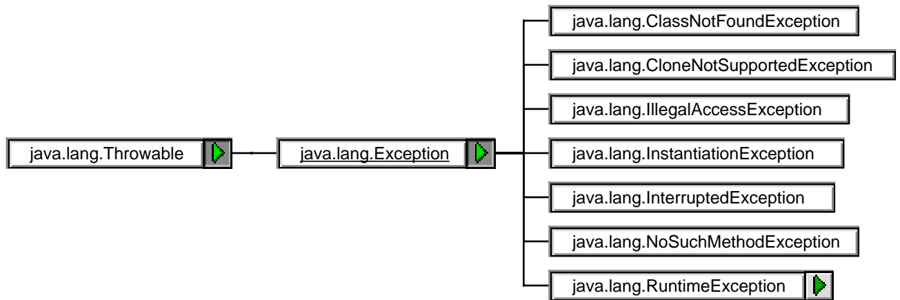
Figure 2.3 An Overview of the java.lang.Exception classes.
