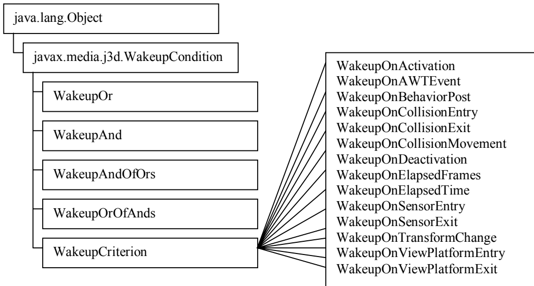
Figure 4-7 The Java 3D API Class Hierarchy for WakeupCondition and Related Classes.
